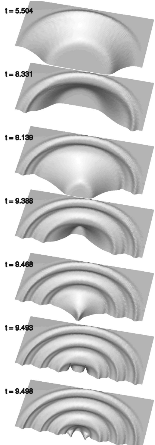
FIG. 2. Several frames of \Phi(\bar{r}, \theta, t) from the evolution of near-critical, \epsilon^2 = 3/4 prolate initial data [Eq. (9)]. Here we have transformed to coordinates \bar{r} = \ln(\sqrt{\rho^2 + z^2} + e_0) - \ln e_0 (with e_0 = 2 \times 10^{-4} ) and \tan \theta = \rho/z , to give a better view of the initial self-similar nature of the solution. [\bar{r}, \theta] ranges from [0 \dots \approx 10.8, 0 \dots \pi] , with the axis \rho=0 being the nearest edge in each figure. The height of each surface represents the magnitude of \Phi . The times shown correspond to the times when \Phi reaches a local minima/maxima, demonstrating the bifurcation that occurs after about two self-similar echoes of the field.
